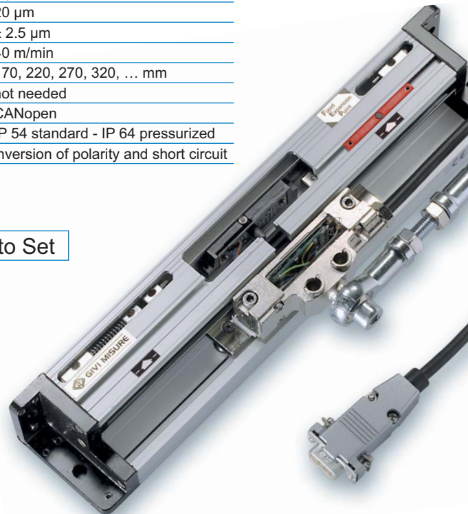
Section of the scale in T-version, SYMMETRIC .
