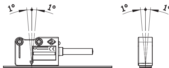
Sensor alignment tolerances.
