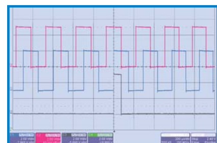
Square-wave output signals from transducer.
