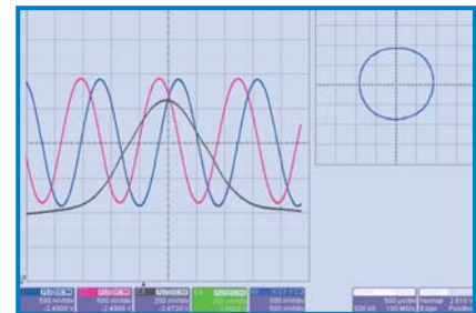
Sine-wave output signals from transducer.
